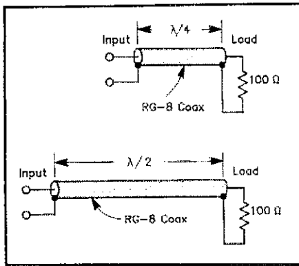
Fig 3—Part of the answer to the problem posed in Fig 2. When the line is \frac{1}{4} \lambda long, it looks like 25 \Omega at the input end when the load is 100 \Omega . When the line is \frac{1}{2} \lambda long, the input end shows an impedance equal to that connected at the load end.
