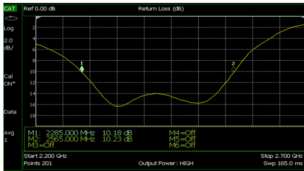
Figure 5a and 5b. Frequency response measurement of a panel antenna showing (a) return loss (dB) and (b) VSWR
