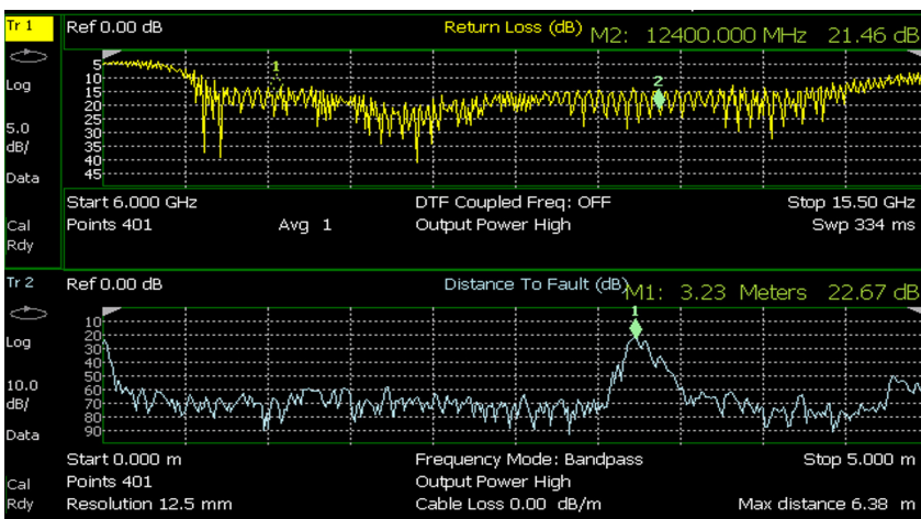
Figure 1. Measured return loss (upper trace) and distance-to-fault (lower trace) for an X-band antenna and coaxial feed cable
