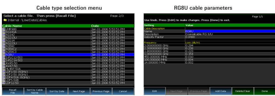
Figure 12. Cable type selection and cable parameter menus on FieldFox
